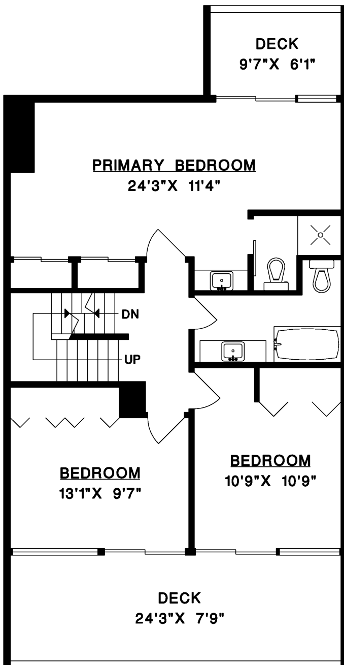
UPPER FLOOR
