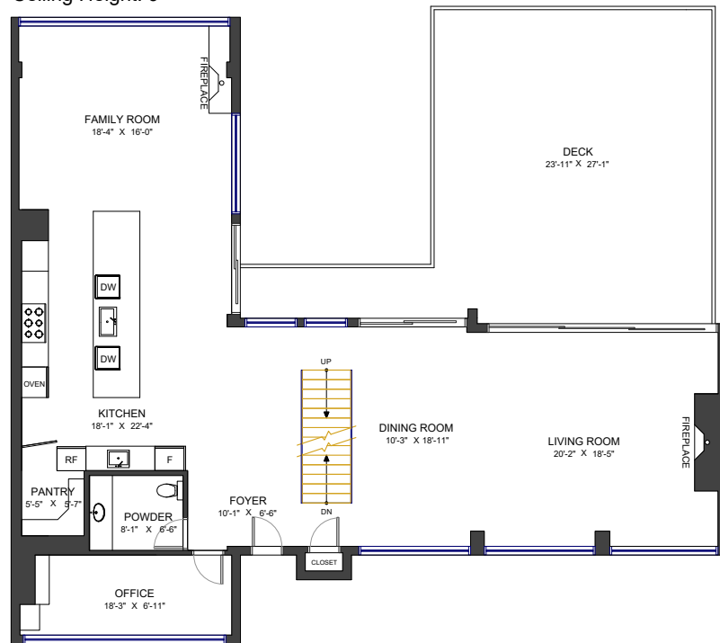
Main Floor Ceiling Height: 9'
