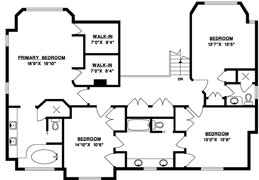
UPPER FLOOR
