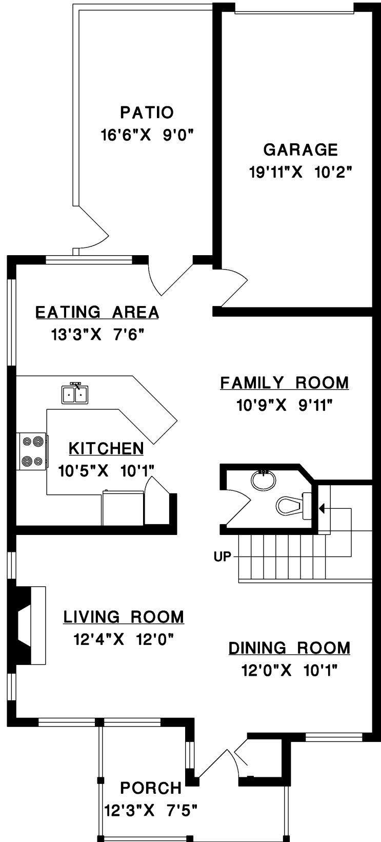
MAIN FLOOR
