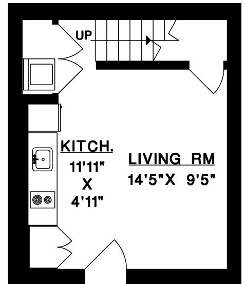
BOTTOM FLOOR
