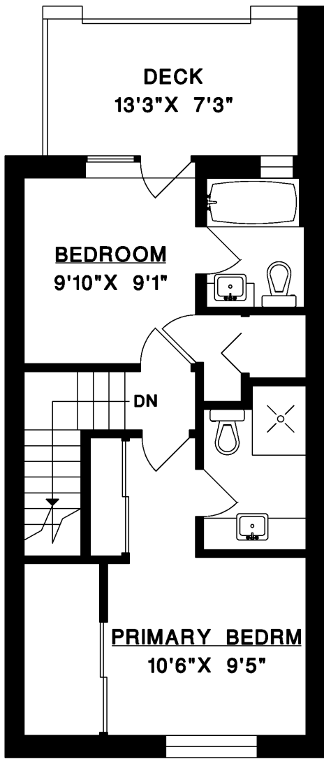
UPPER FLOOR
