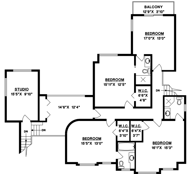
UPPER FLOOR
