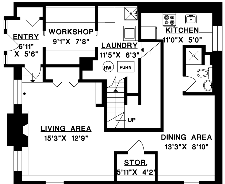
LOWER FLOOR
