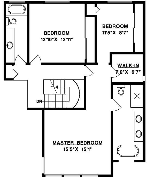
UPPER FLOOR
