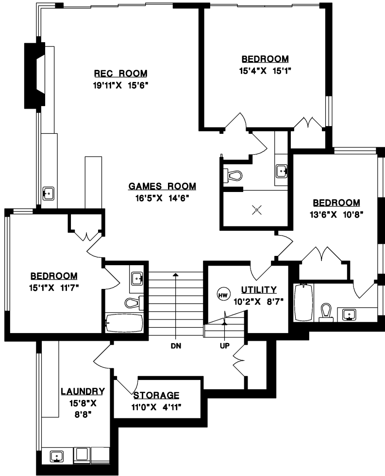
LOWER FLOOR
