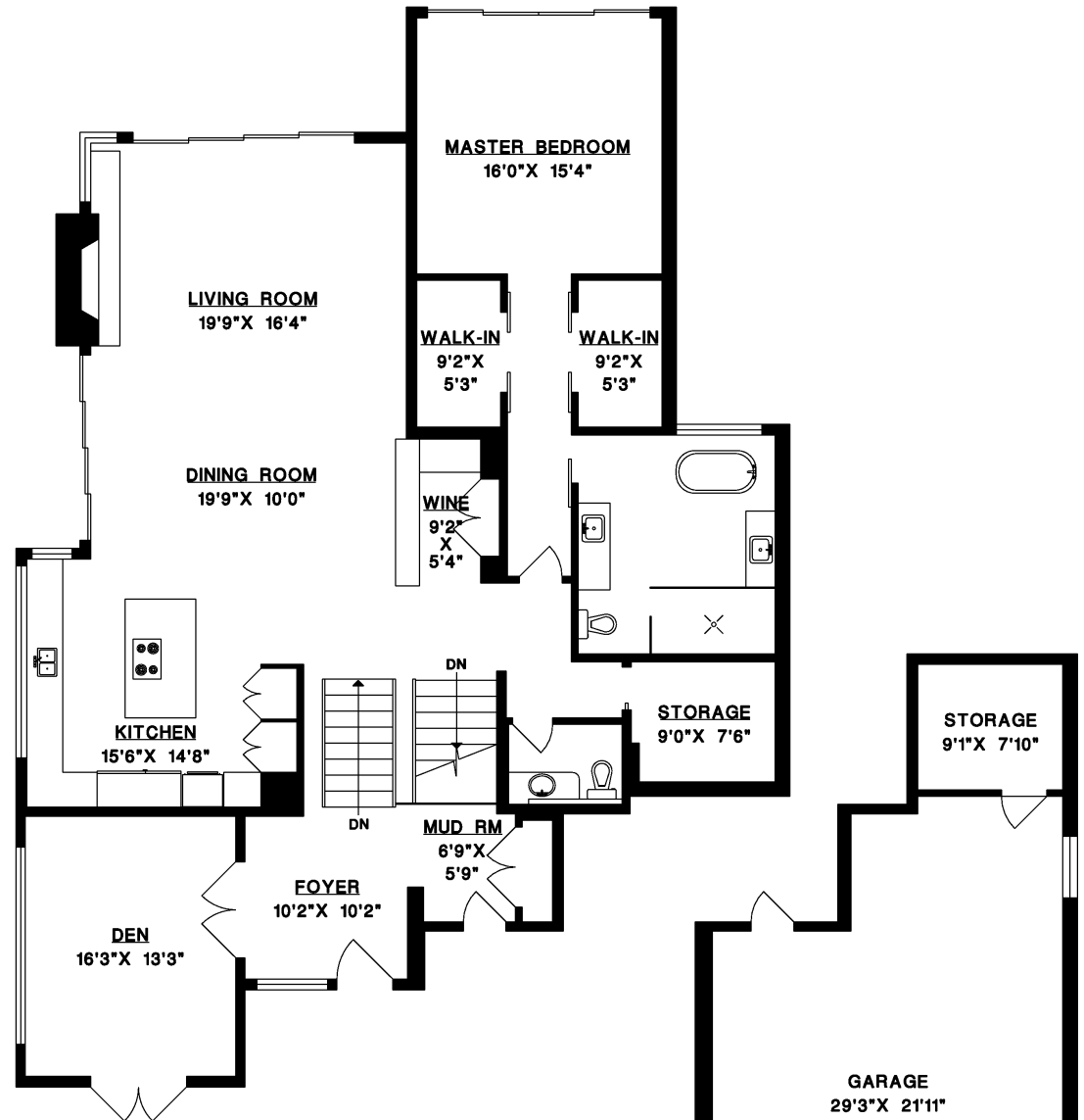
MAIN FLOOR
